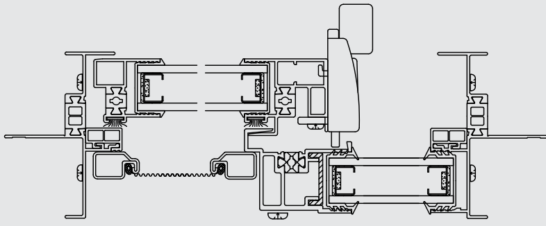
Horizontal Detail
