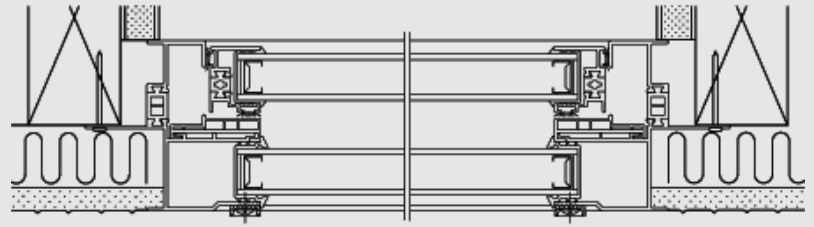
Single Hung Detail
